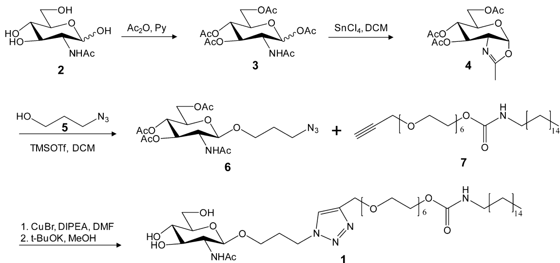
Fig. 2 Synthesis of GlcNAc-alkyl. A facile and scalable eight-step process is followed to produce the tethering and targeting compound GlcNAc-alkyl. During nanoparticle production, the hydrophobic alkyl
