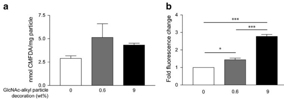
Fig. 4 Measurement of particle internalization by CMFDA fluorescence demonstrating increased uptake. PK-GlcNAc-CMFDNA nanoparticles were decorated with 0%, 0.6%, or 9% GlcNAc-alkyl by weight and loaded with the cell tracker dye, 5-chloromethylfluorescein diacetate (CMFDA). a Particles are closely load-matched for CMFDA content: 0%, 0.6%, and 9% decorated particles contained 2.9±0.3, 5.1 ±1.5, and 4.3±0.2 nmol CMFDA/mg particle, respectively. Data are expressed as mean±SEM from three experiments. b After incubation
