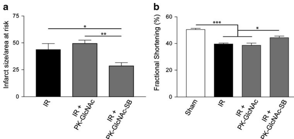
Fig. 7 Infarct size reduction and functional improvements seen in PK-GlcNAc-SB treatment following ischemia–reperfusion injury. Immediately following IR, particles were injected directly into the injured myocardium. Three days following surgery, echocardiography was performed and heart cross sections analyzed for infarct size. a The ratio of infarct size to area at risk was calculated for the treatment groups. PK-GlcNAc treatment had no significant effect, but PK-GlcNAc-SB treatment significantly decreased infarct size compared to both treatment groups (mean \pm SEM, n=5 ; *p<0.05 , **p<0.01 ;
