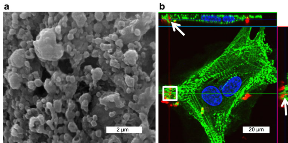
Fig. 3 Incubation of CMs with PK-GlcNAc-rhodamine particles for internalization verification. a Rhodamine-loaded particles (diameter= 320 \pm 156 nm) were decorated with GlcNAc-alkyl and imaged by SEM. b Cultured CMs were treated with PK-GlcNAc-rhodamine particles for 12 h before fixation in paraformaldehyde and immunostaining for
