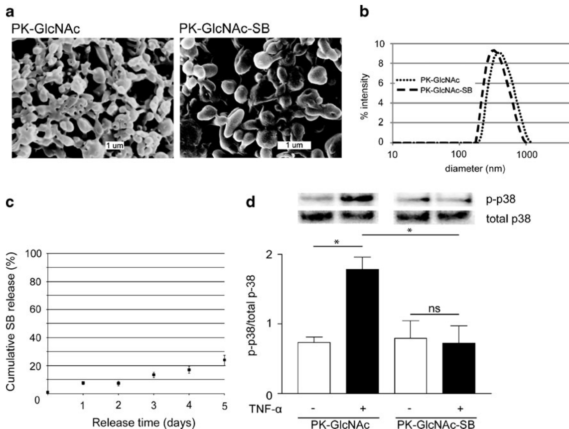
Fig. 5 Treatment of CMs in vitro with p38 inhibitor-loaded nanoparticles reduces TNF-α-stimulated p38 activation. PK-GlcNAc and PK-GlcNAc-SB particles were imaged via a SEM (diameter=407±125 nm or diameter=342±165 nm, respectively) and b analyzed by DLS (diameter=465±173 nm or diameter=395±145 nm, respectively). Data are mean±SD. c PK-GlcNAc-SB particles release cargo through
